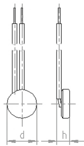
Installation height h from 5,0 mm Diameter d 11,0 mm
